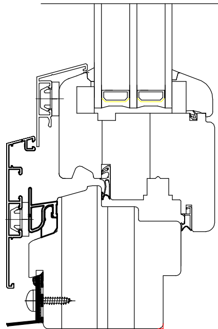
A A-1 Tilt-Turn Window - Vertical Section
